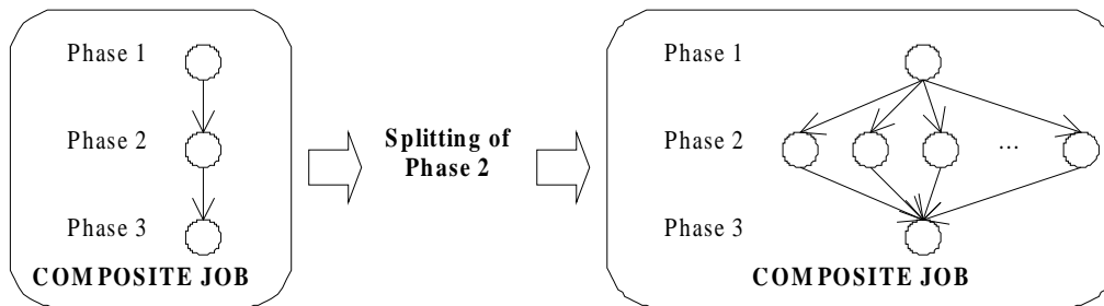
Figure 8: An example illustrating both processing chains (left panel) and job splitting (right panel).
